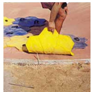
4 The patterned finish is created by placing the mats on the surface of the coloured concrete whilst it is still in its 'wet' state. The CCS stamping mats can also be used on fresh, integrally coloured concrete.
